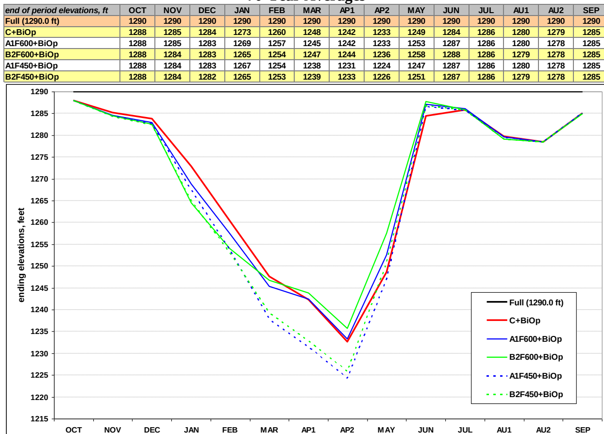
Figure C-6 Grand Coulee Elevations, feet - Supplemental Studies 70-Year Averages
