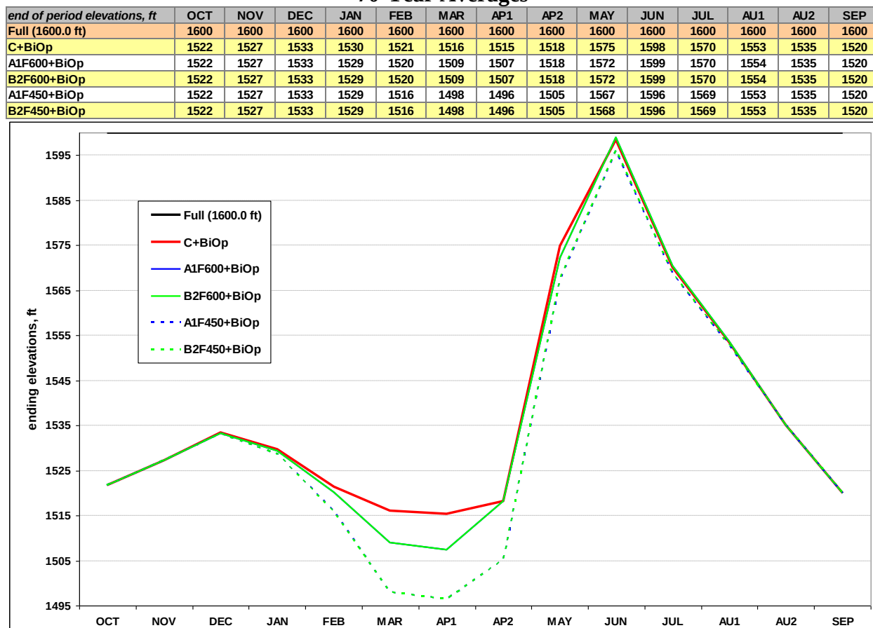
Figure C-9 Dworshak Elevations, feet - Supplemental Studies 70-Year Averages
