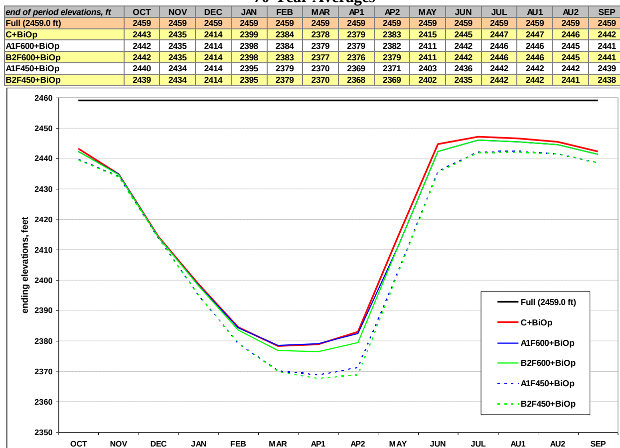
Figure C-7 Libby Elevations, feet - Supplemental Studies 70-Year Averages
