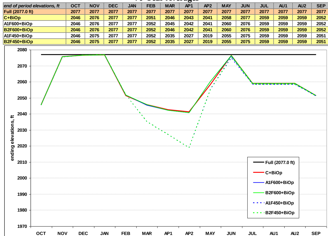
Figure C-10 Brownlee Elevations, feet - Supplemental Studies 70-Year Averages
