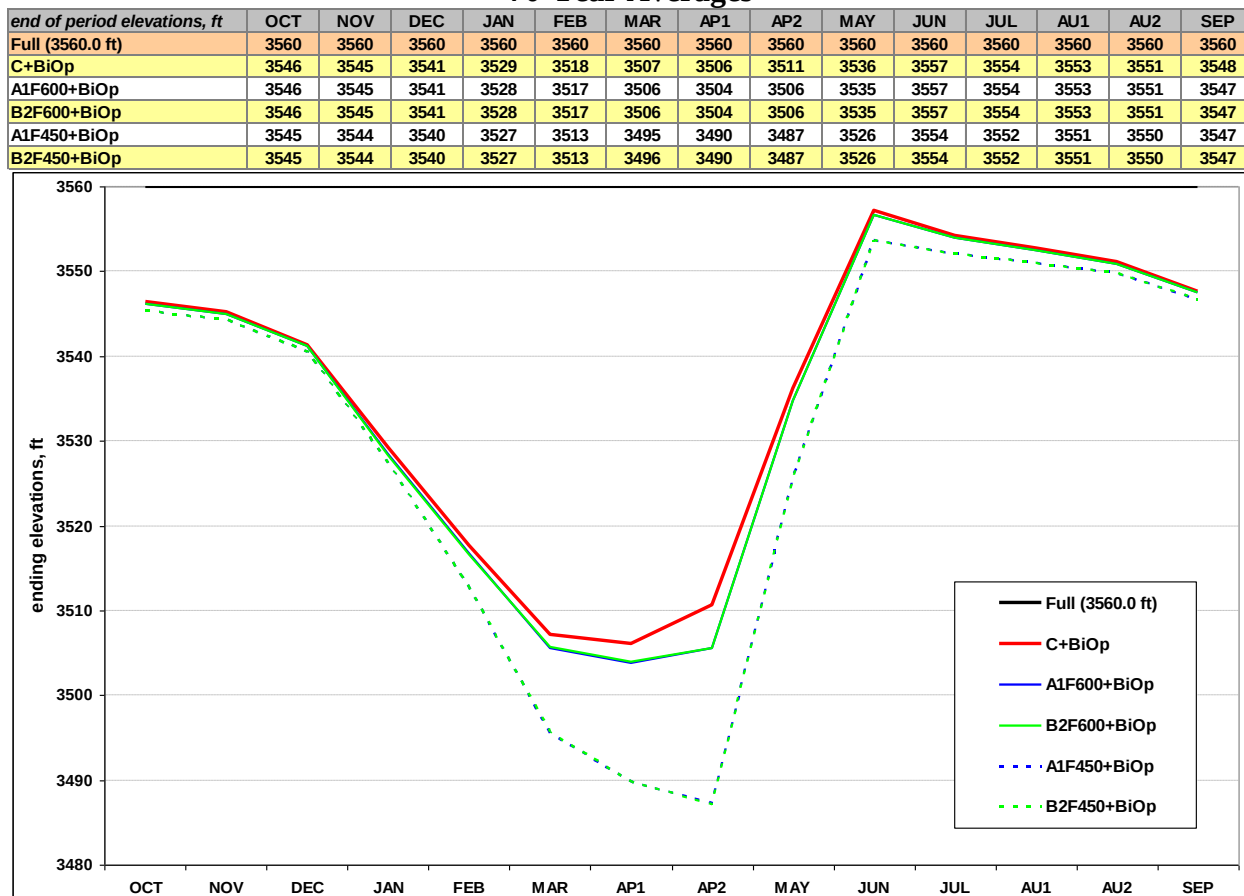
Figure C-8 Hungry Horse Elevations, feet - Supplemental Studies 70-Year Averages
