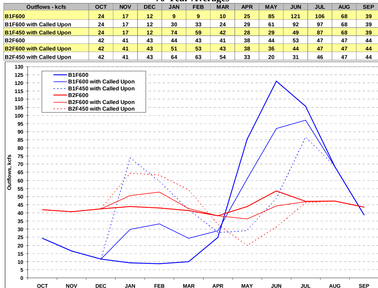
Figure 3 - Arrow plus Duncan Outflows – B1 vs. B2 Scenarios 70-Year Averages
