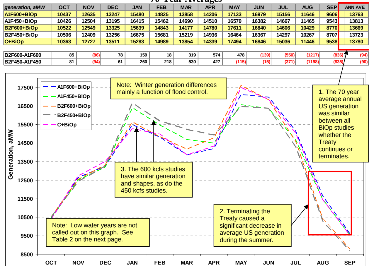
Figure 6 - U.S. System Generation - Supplemental Studies 70-Year Averages
