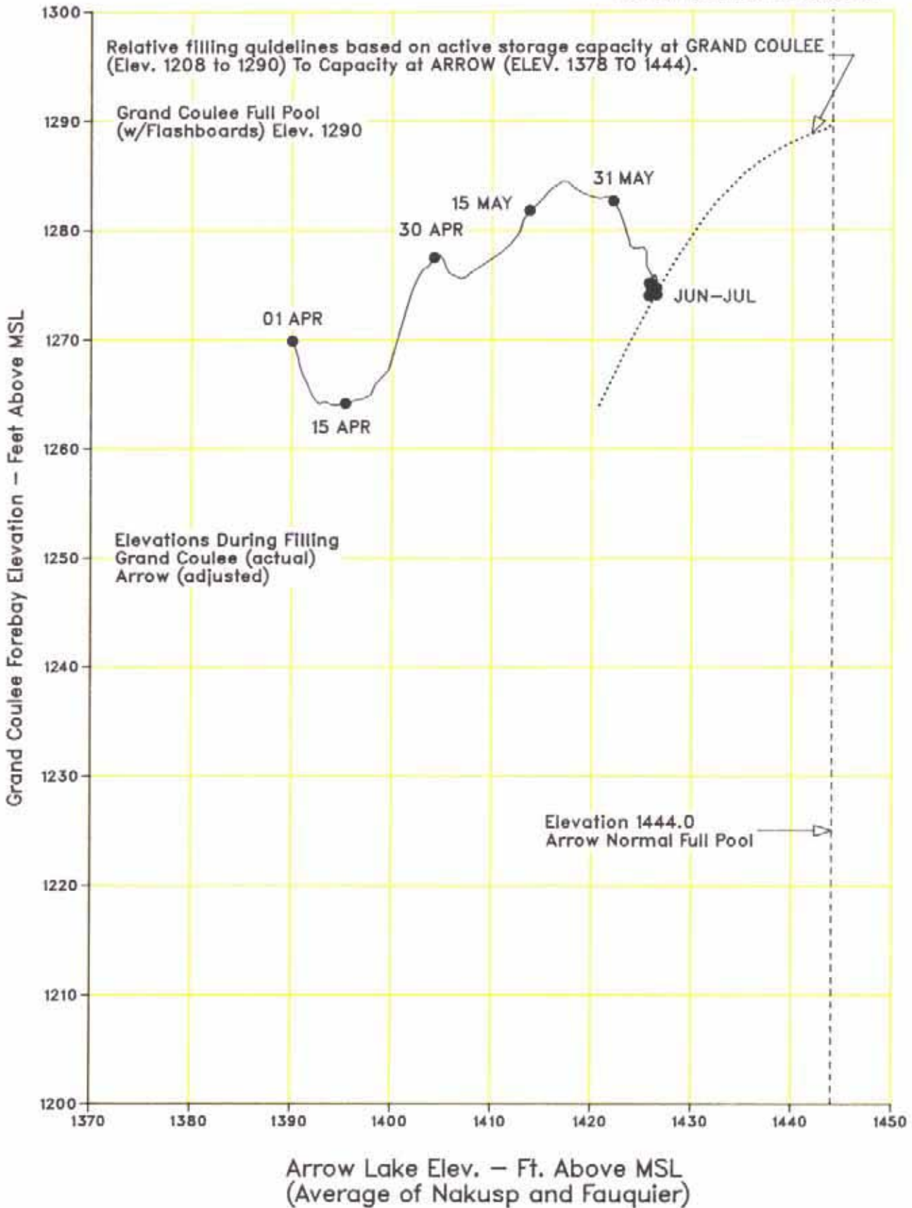
Chart 15 1994 Relative Filling Arrow and Grand Coulee
