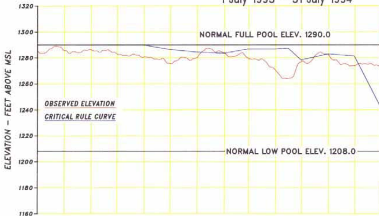
Chart 12 Regulation of Grand Coulee 1 July 1993 – 31 July 1994
