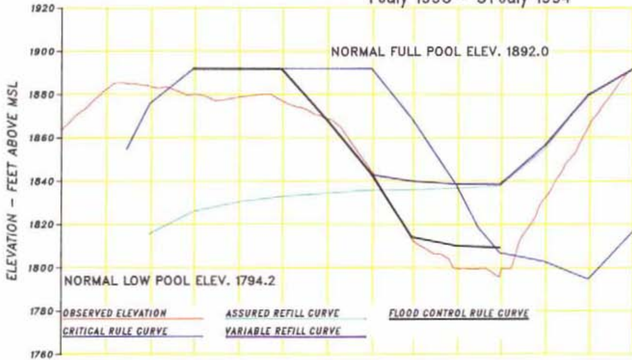
Chart 8 Regulation of Duncan 1 July 1993 – 31 July 1994
