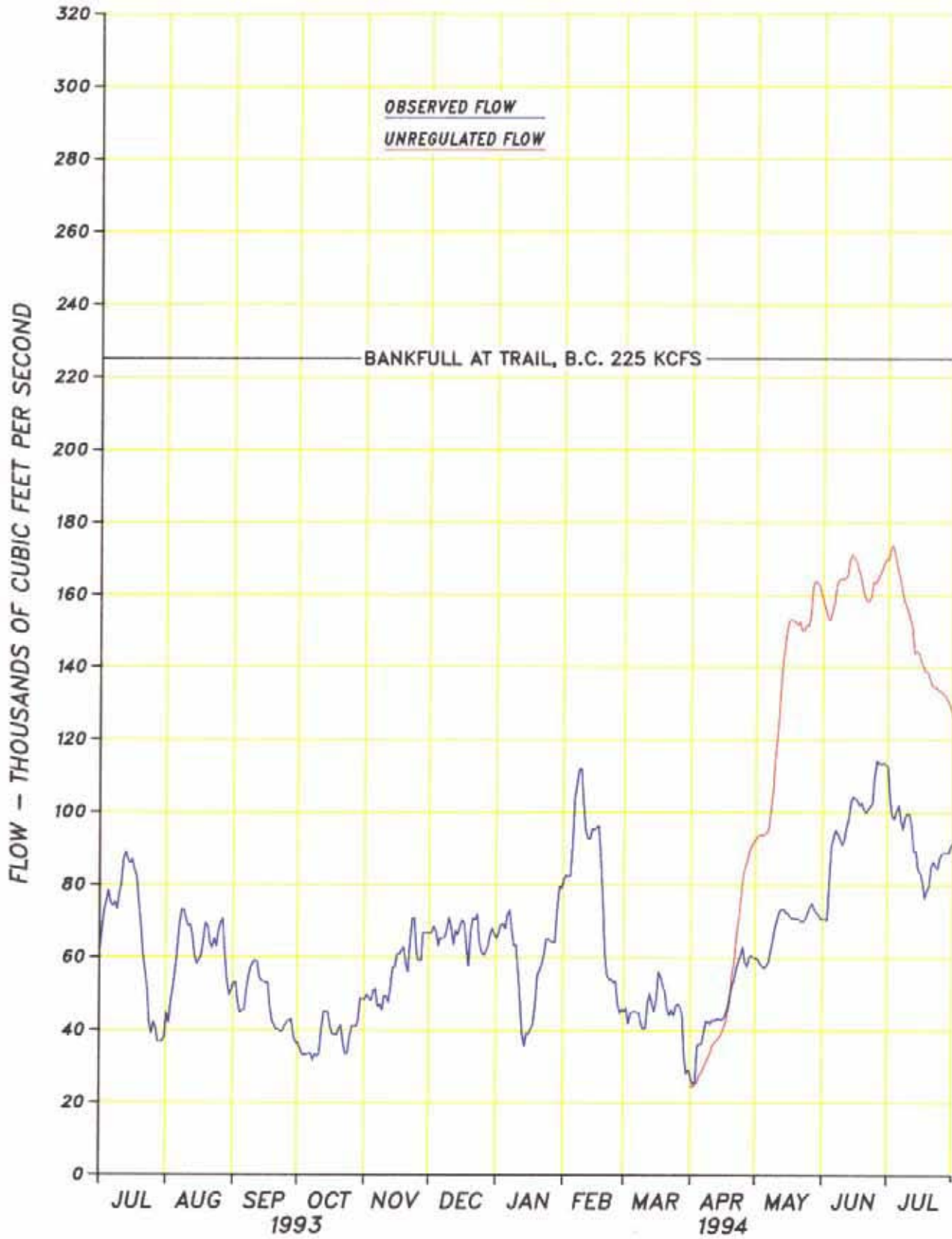
Chart 11 Columbia River at Birchbank 1 July 1993 - 31 July 1994
