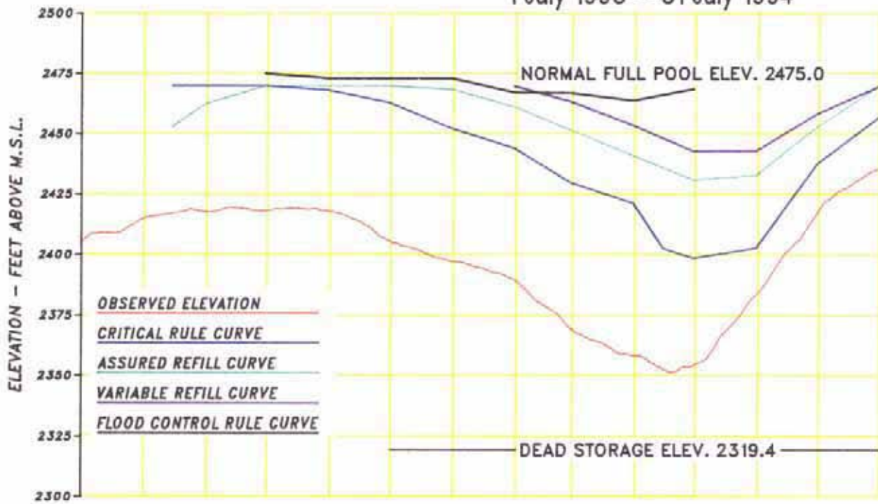
Chart 6 Regulation of Mica 1 July 1993 – 31 July 1994
