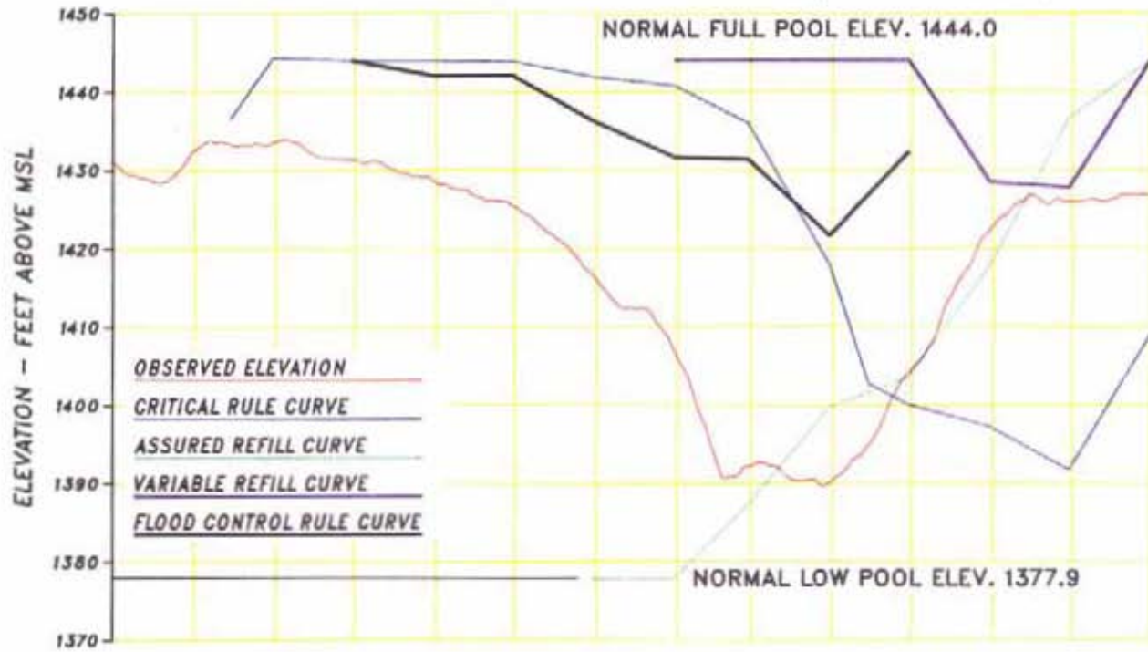
Chart 7 Regulation of Arrow 1 July 1993 – 31 July 1994
