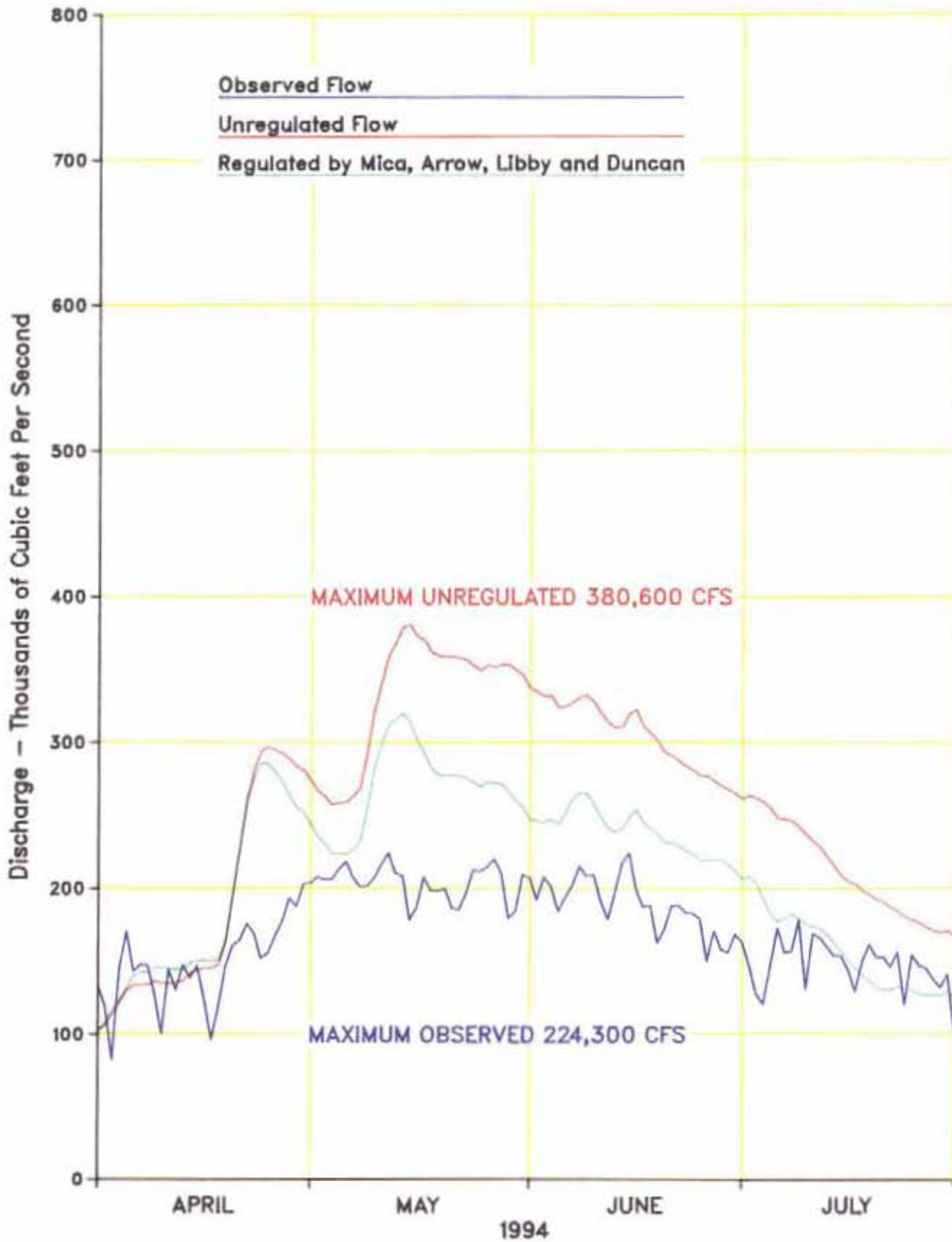
Chart 14 Columbia River at The Dalles 1 April 1994 - 31 July 1994
