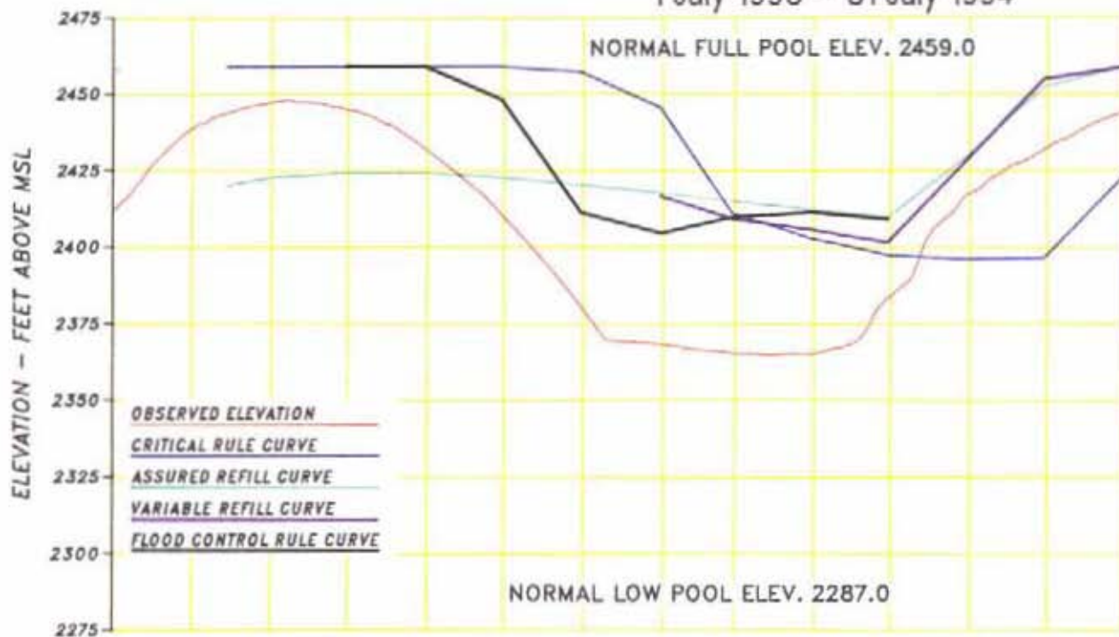
Chart 9 Regulation of Libby 1 July 1993 – 31 July 1994
