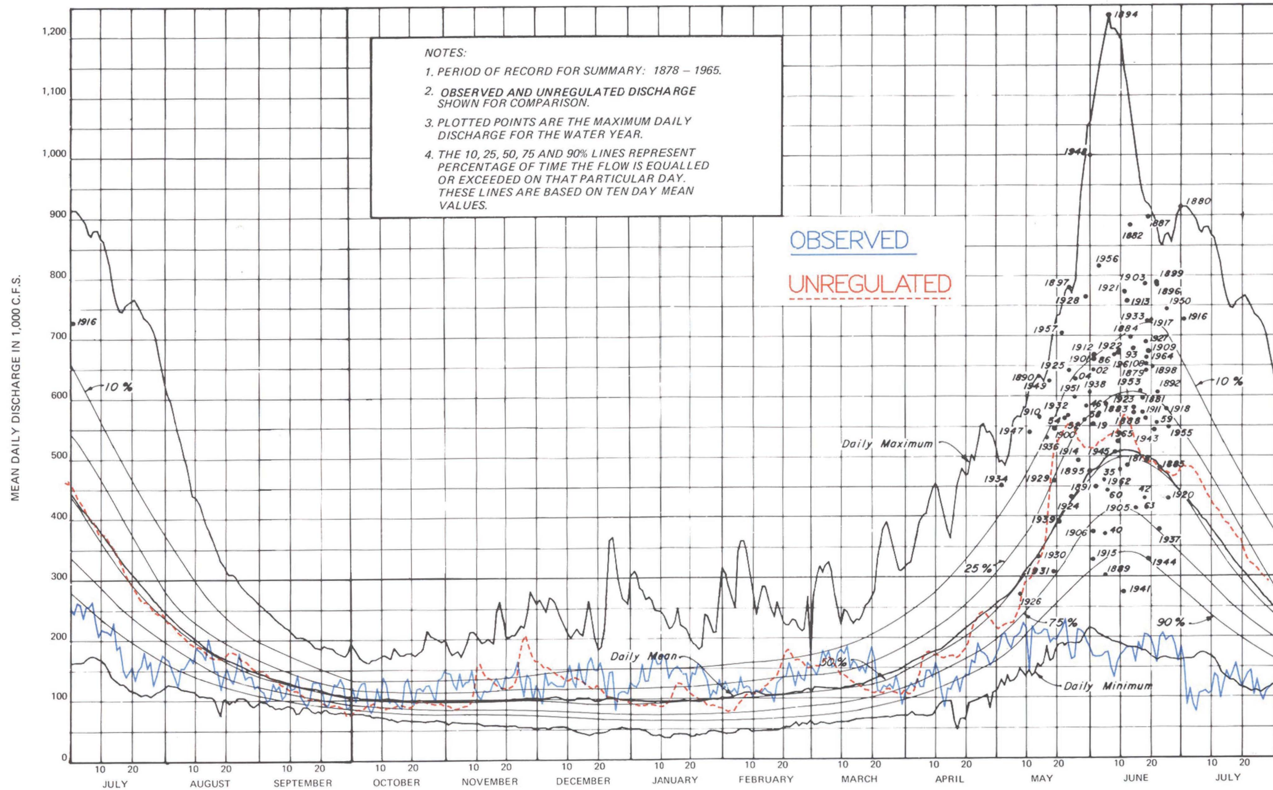
Chart 13 Columbia River at The Dalles 1 July 1991 - 31 July 1992
