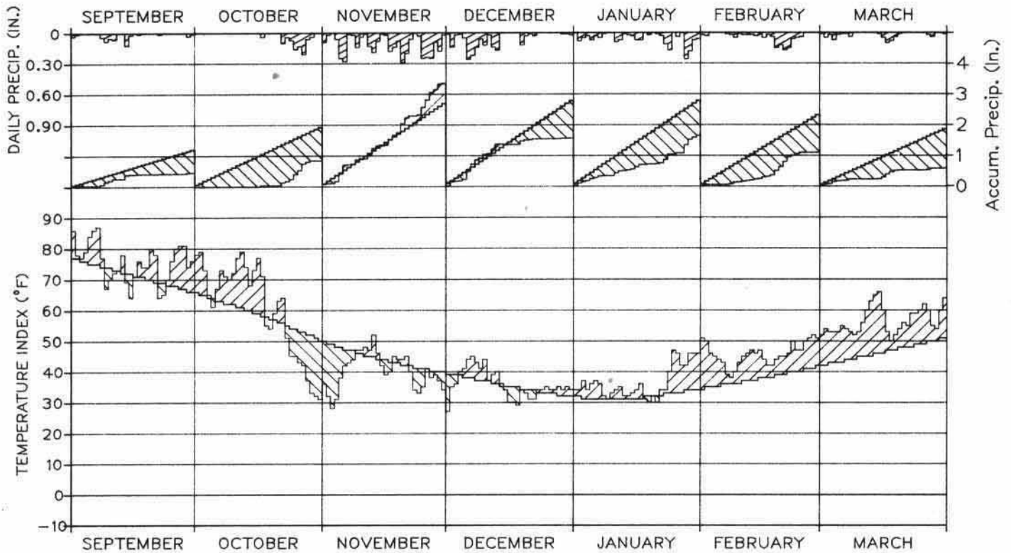
Chart 3 WINTER SEASON TEMPERATURE AND PRECIPITATION INDEX 1991-1992 Columbia River Basin Above The Dalles, OR
