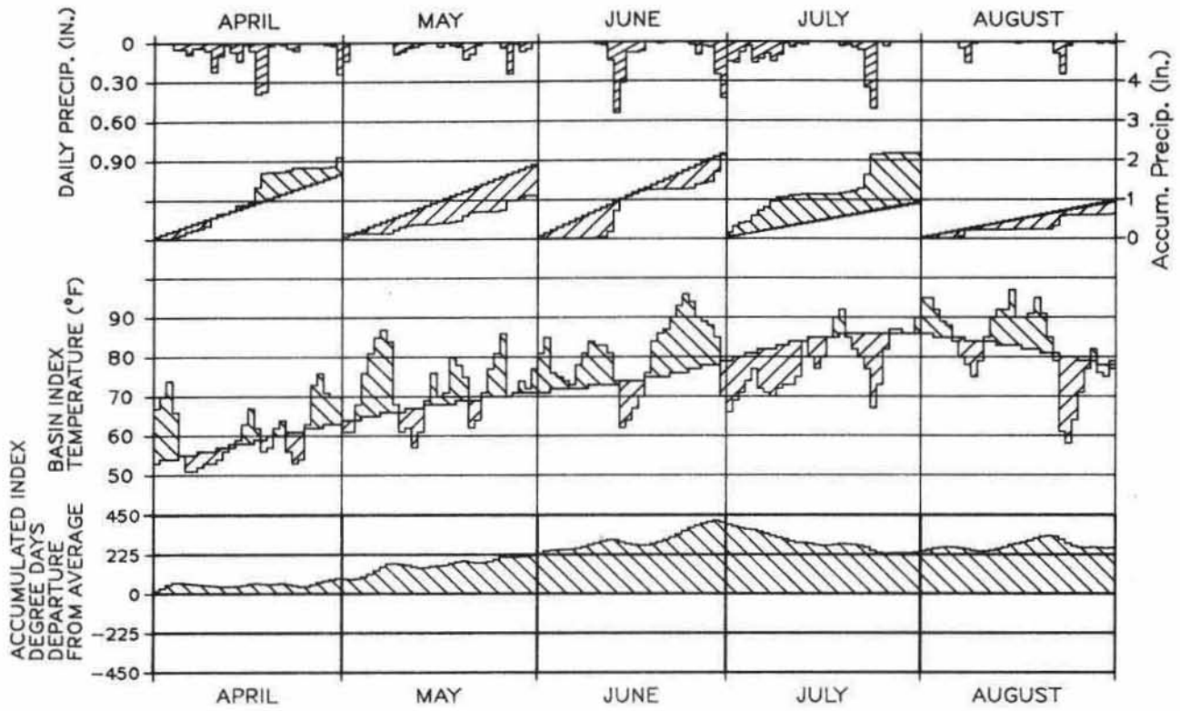
1992 SNOWMELT SEASON CHART 4 TEMPERATURE AND PRECIPITATION INDEX Columbia River Basin Above The Dalles, OR
