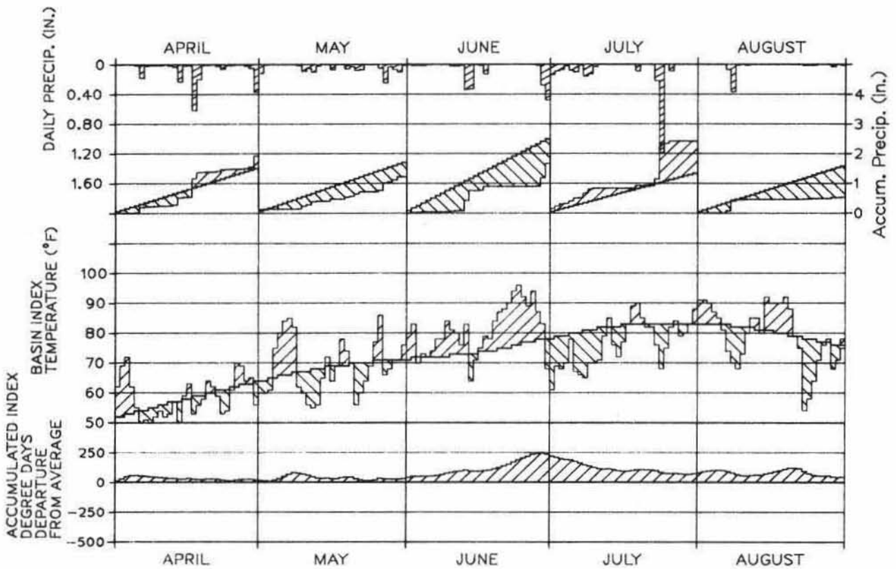
1992 SNOWMELT SEASON Chart 5 TEMPERATURE AND PRECIPITATION INDEX Columbia River Basin In Canada
