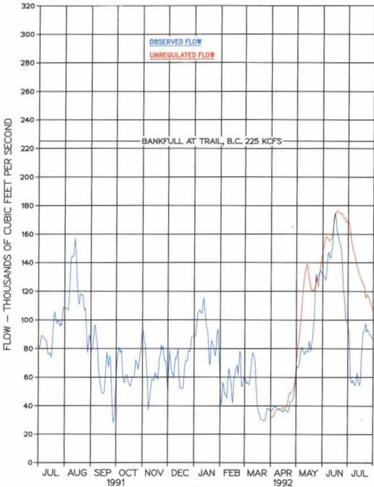
Chart 11 Columbia River at Birchbank 1 July 1991 - 31 July 1992
