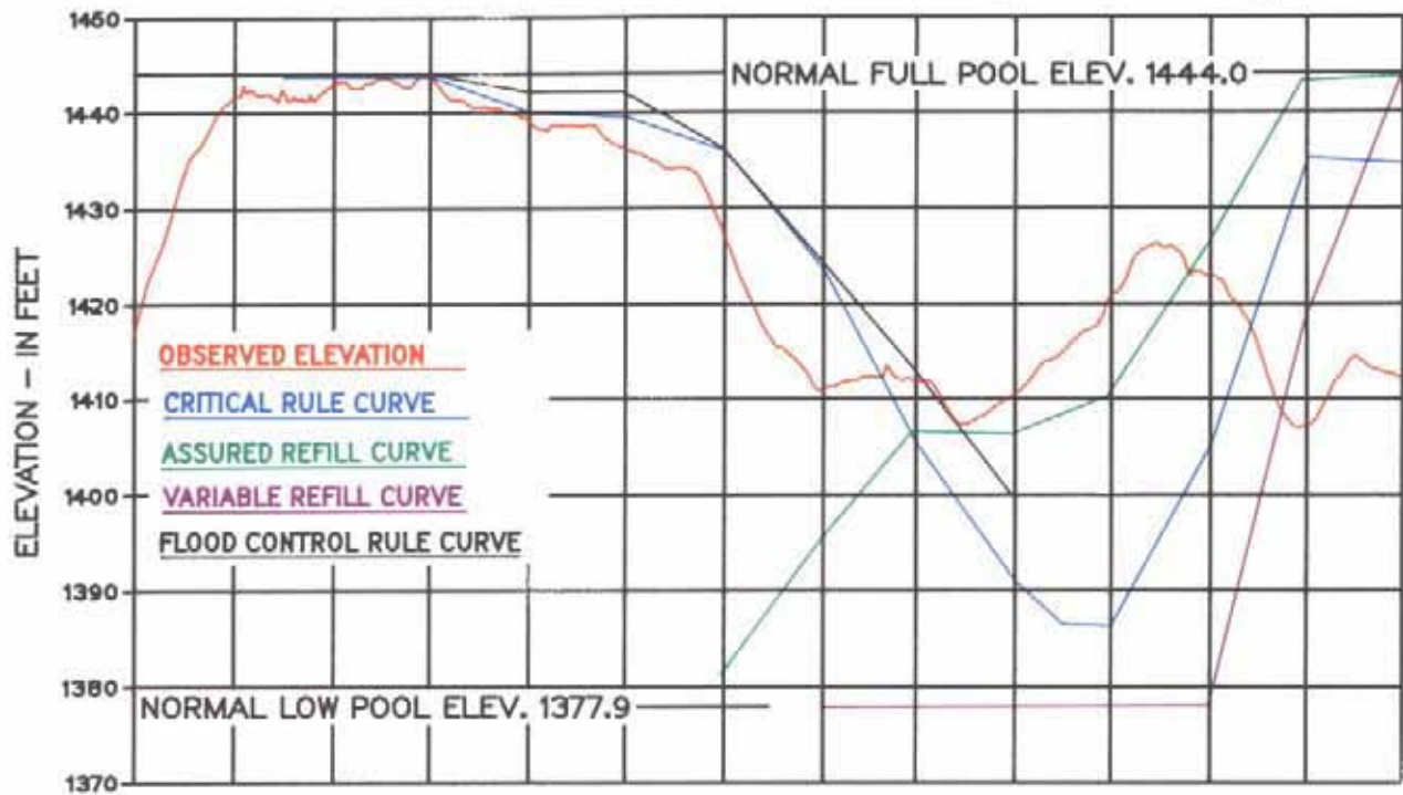
Chart 7 Regulation of Arrow 1 July 1991 – 31 July 1992
