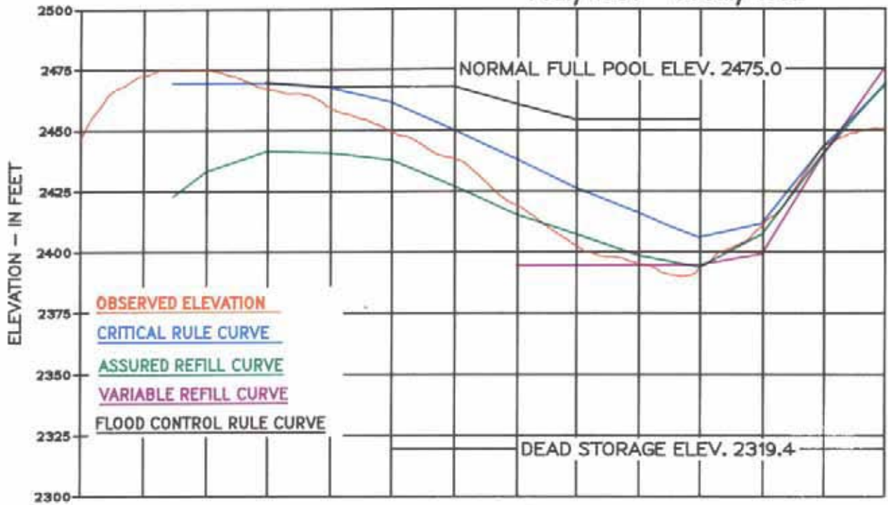
Chart 6 Regulation of Mica 1 July 1991 – 31 July 1992
