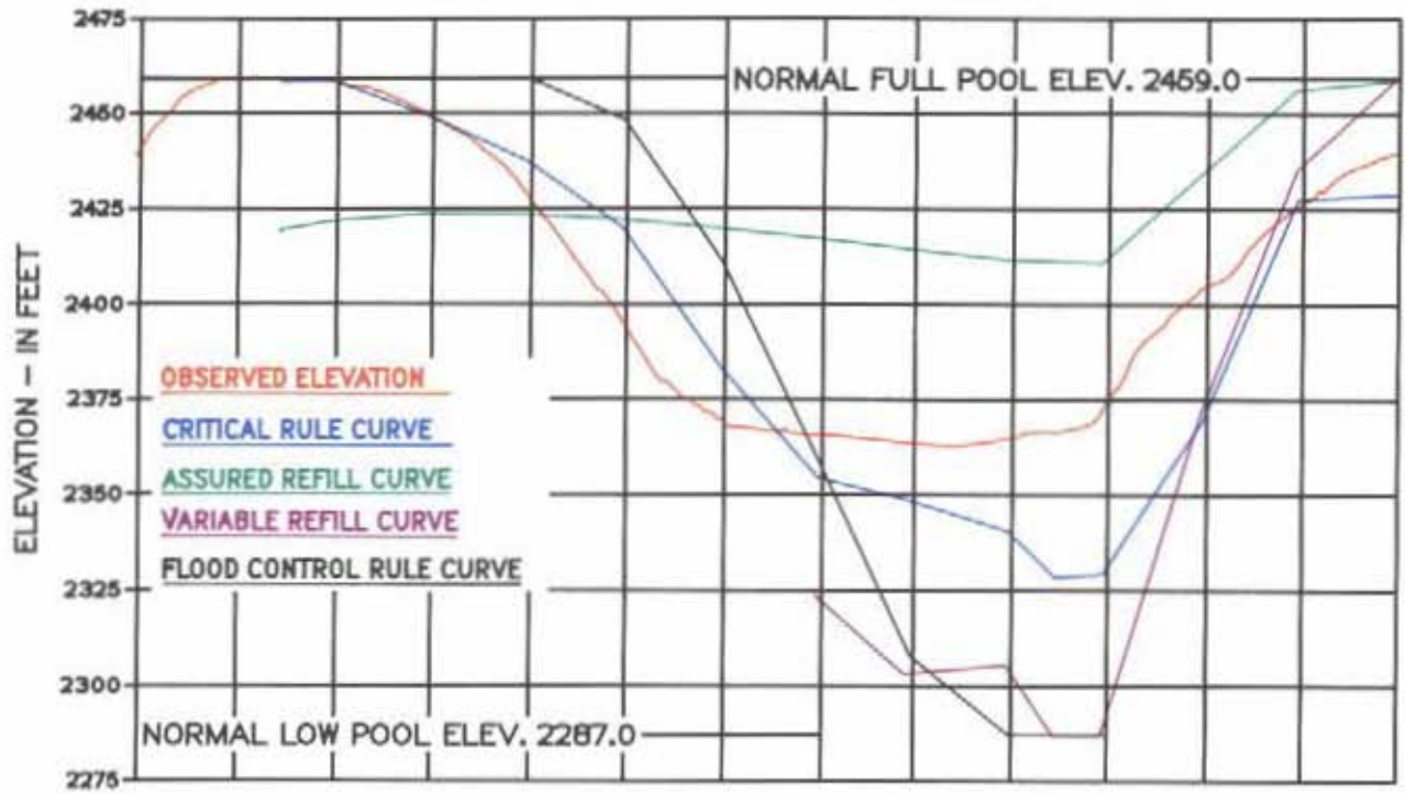
Chart 9 Regulation of Libby 1 July 1991-31 July 1992
