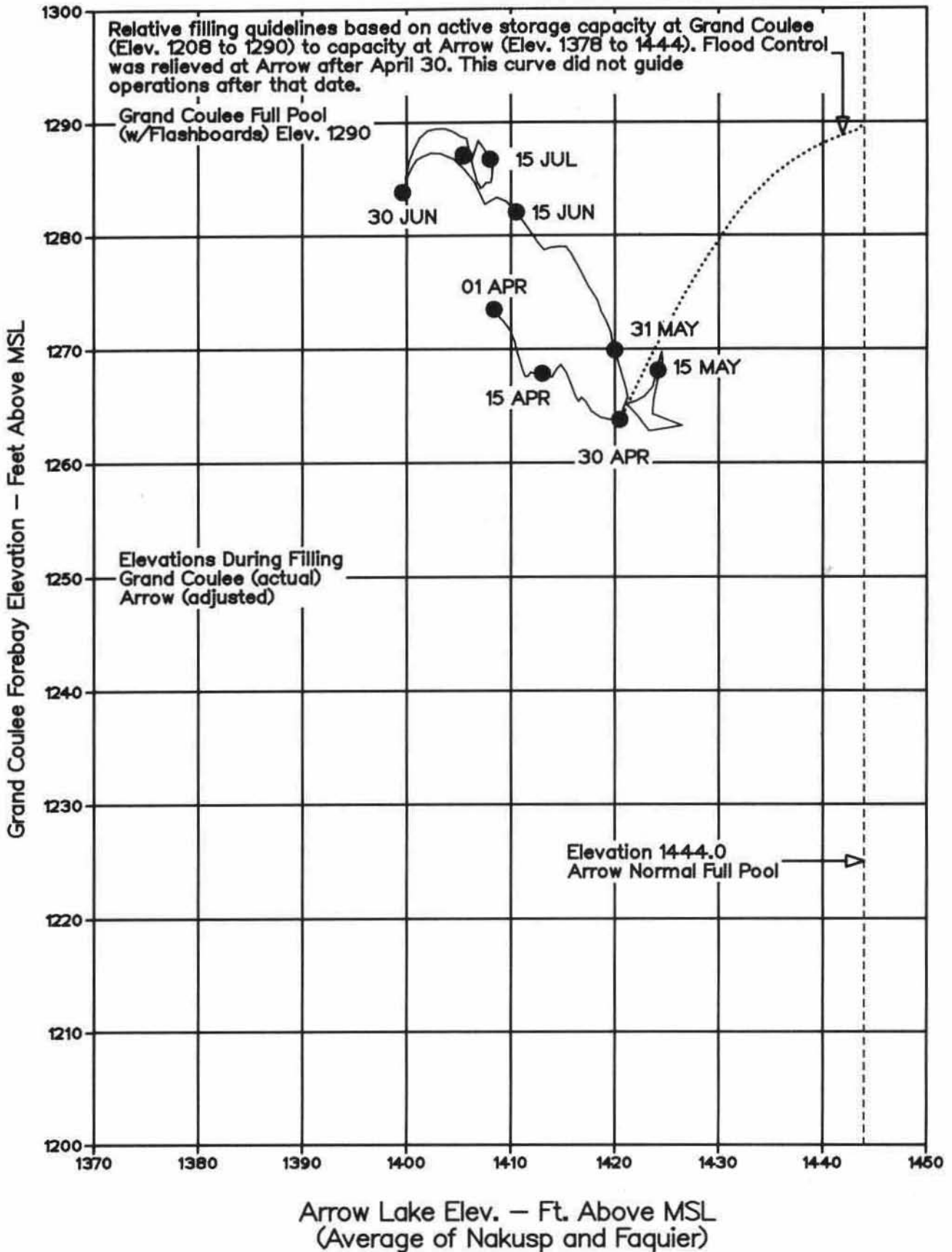
Chart 15 1992 Relative Filling Arrow and Grand Coulee
