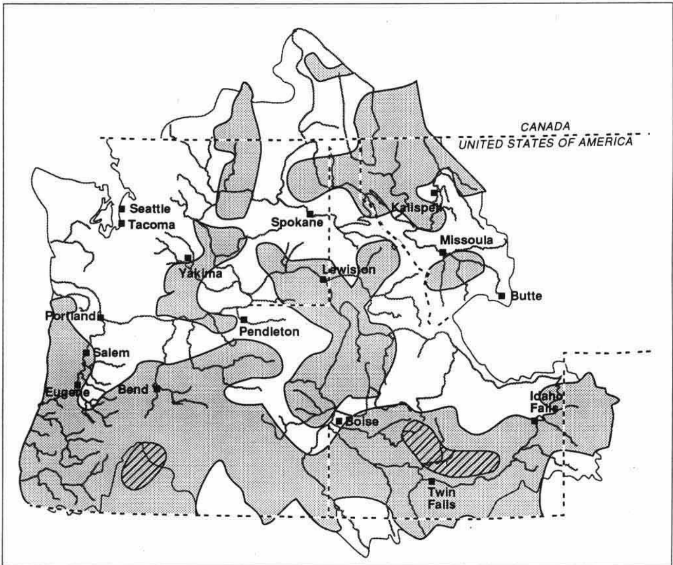
Chart 1 Seasonal Precipitation Columbia River Basin October 1991 - March 1992 Percent of 1961 - 1990 Average
