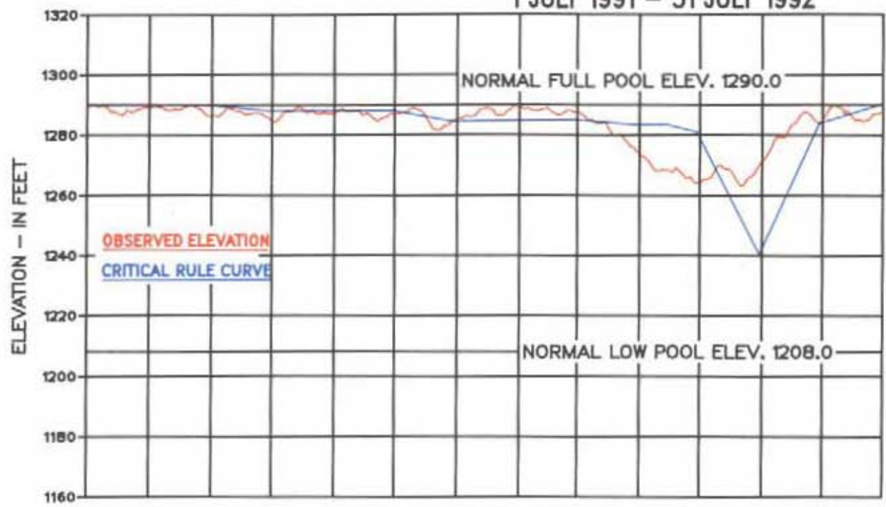
Chart 12 Regulation of Grand Coulee 1 JULY 1991 – 31 JULY 1992
