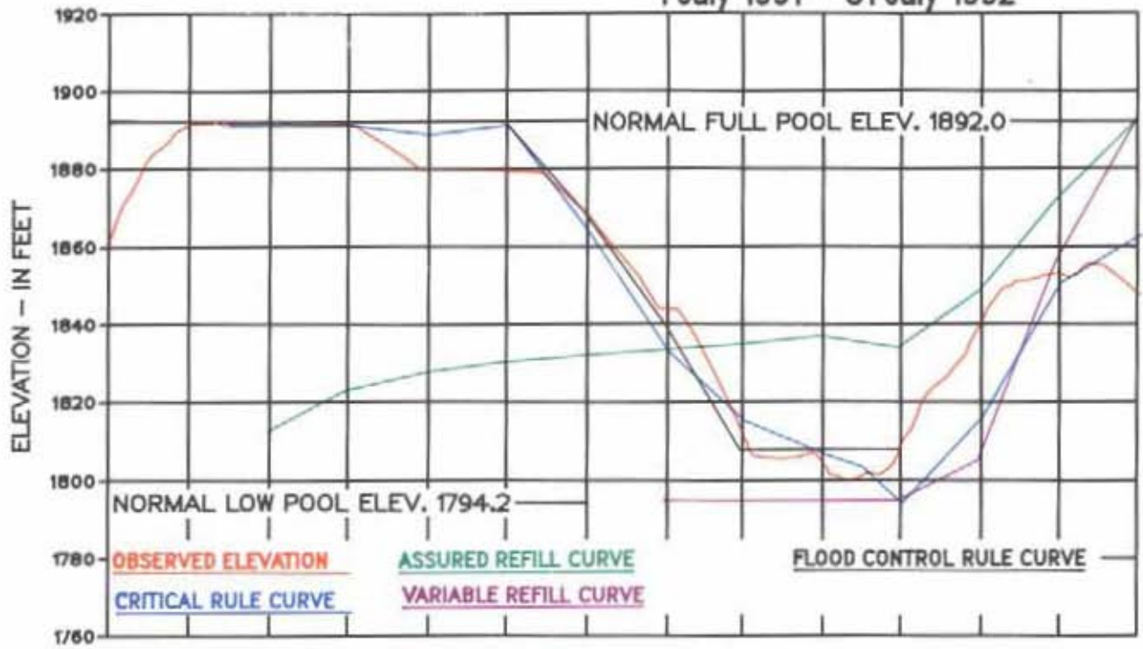
Chart 8 Regulation of Duncan 1 July 1991 – 31 July 1992
