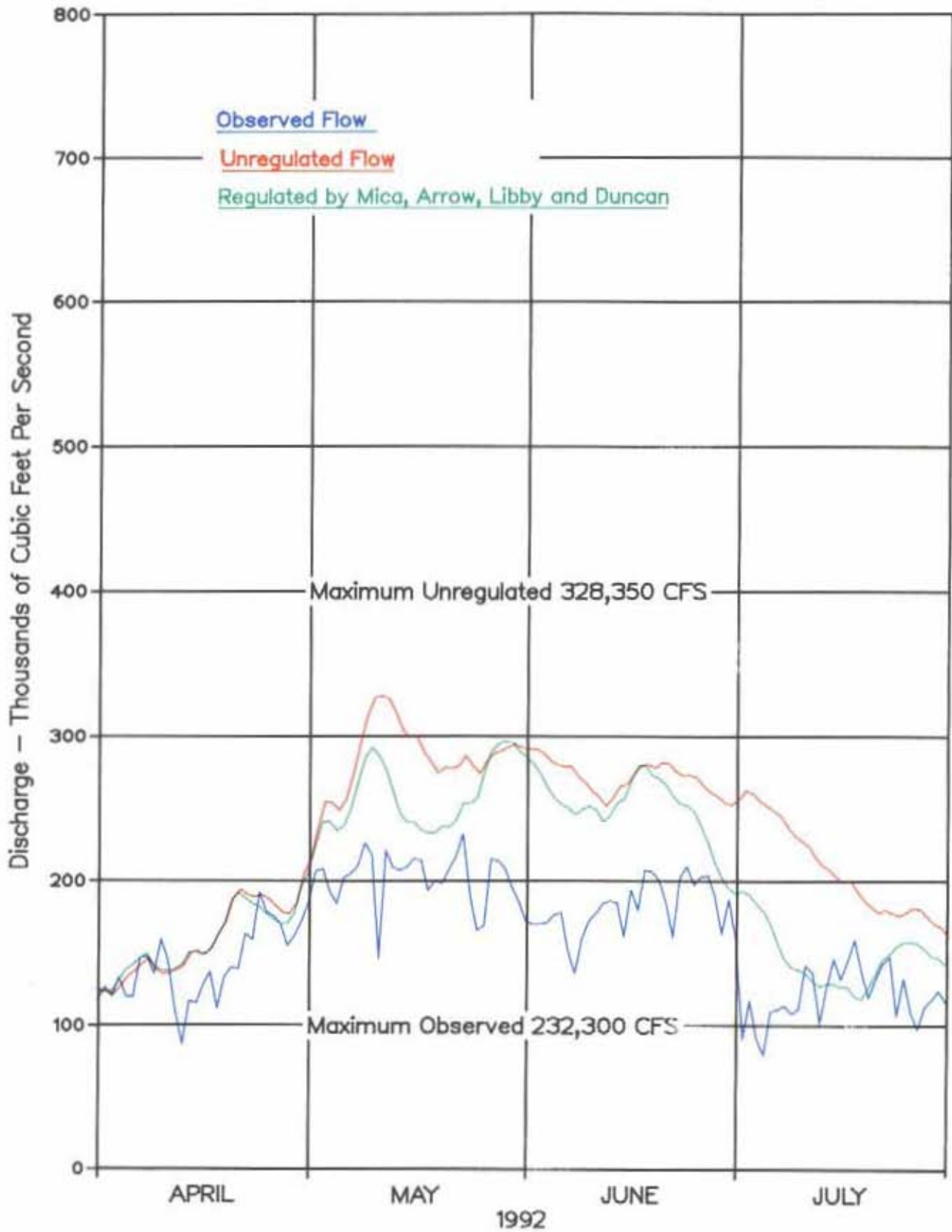
Chart 14 Columbia River at The Dalles 1 April 1992 - 31 July 1992
