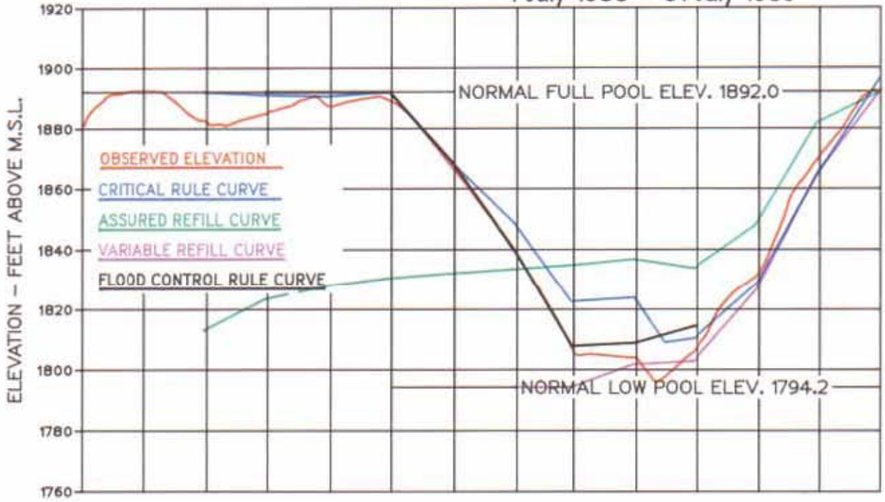
Chart 8 Regulation of Duncan 1 July 1988 – 31 July 1989
