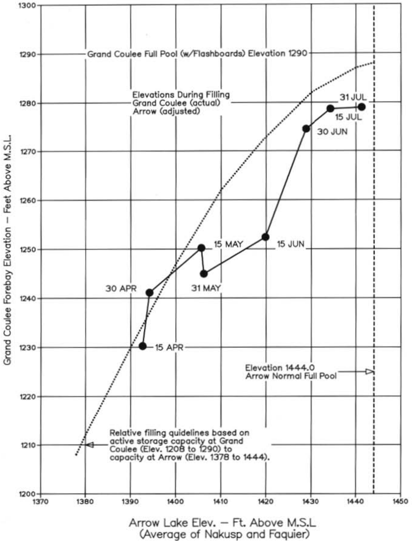
Chart 15 1989 Relative Filling Arrow and Grand Coulee
