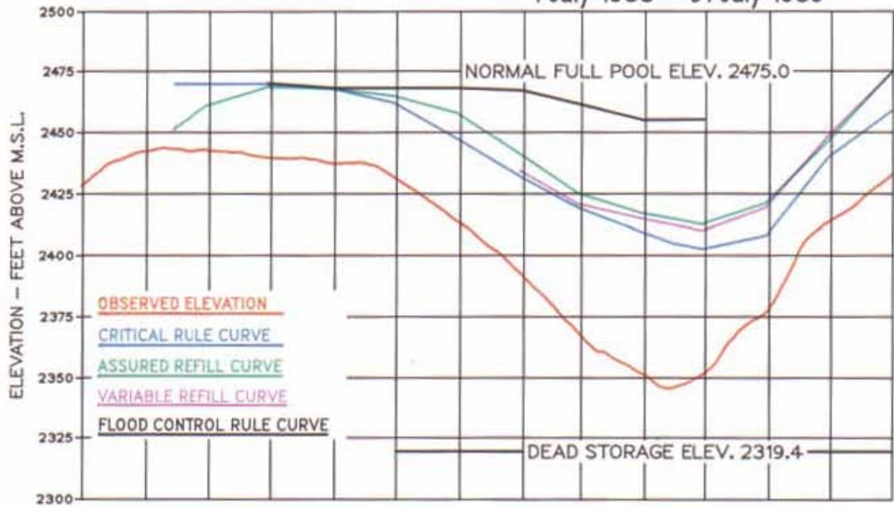
Chart 6 Regulation of Mica 1 July 1988 – 31 July 1989
