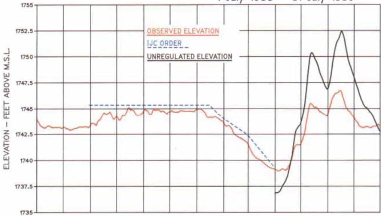
Chart 10 Regulation of Kootenay Lake 1 July 1988 – 31 July 1989
