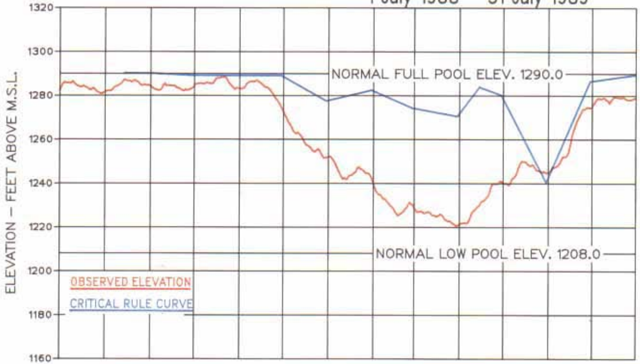
Chart 12 Regulation of Grand Coulee 1 July 1988 – 31 July 1989
