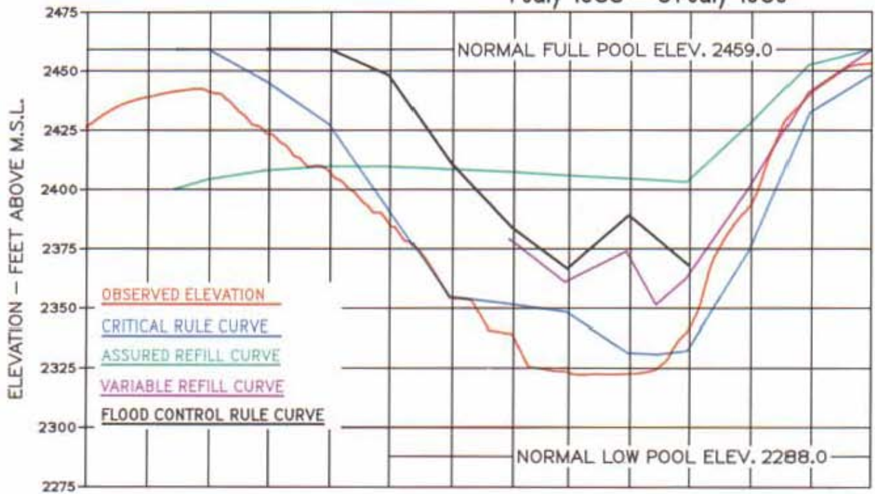
Chart 9 Regulation of Libby 1 July 1988 – 31 July 1989
