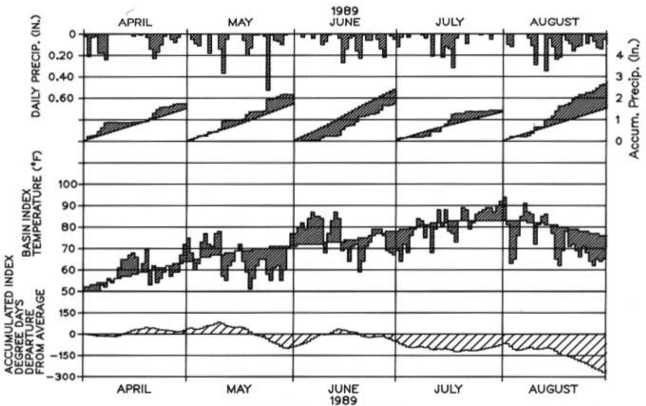
SNOWMELT SEASON Chart 5 Temperature and Precipitation Index 1988-1989 Columbia River Basin In Canada
