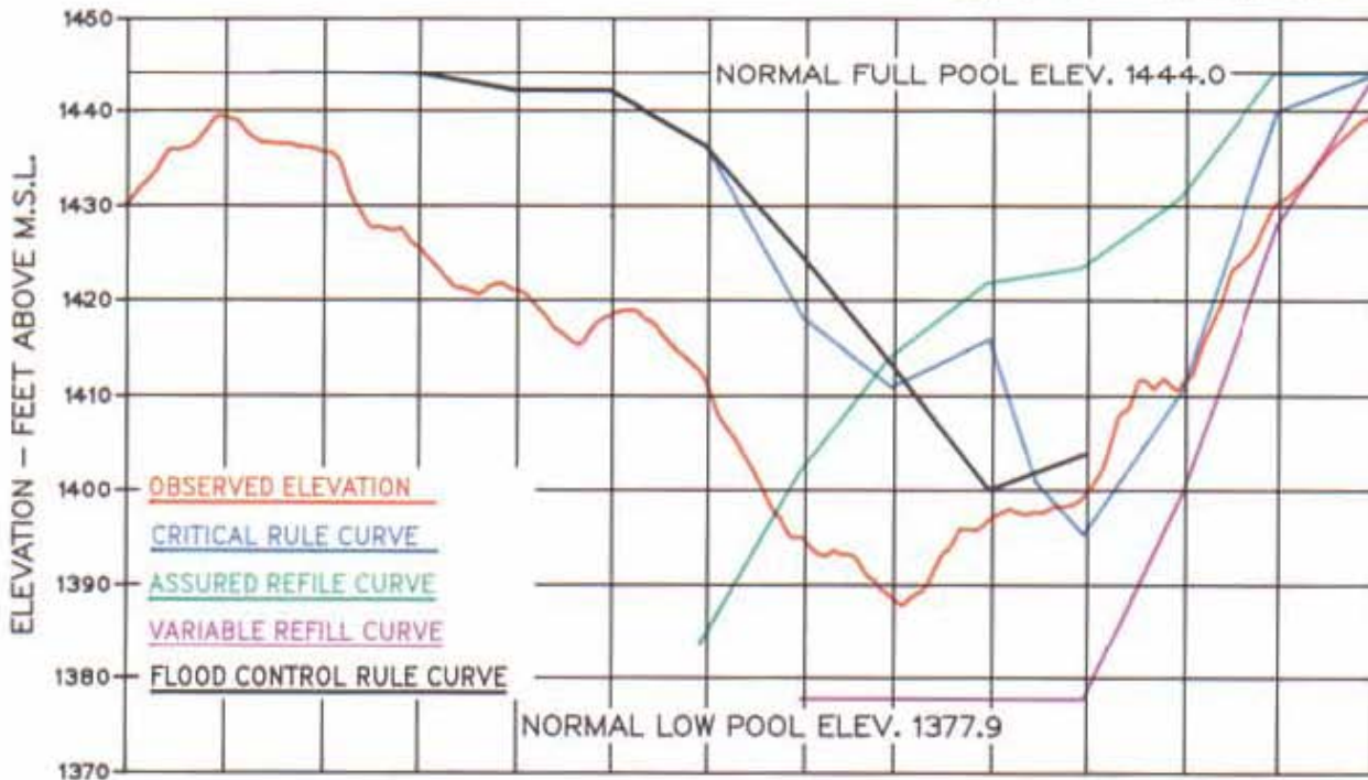
Chart 7 Regulation of Arrow 1 July 1988 – 31 July 1989
