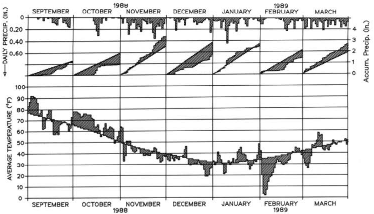
WINTER SEASON Chart 3 Temperature and Precipitation Index 1988-1989 Columbia River Basin Above The Dalles, OR
