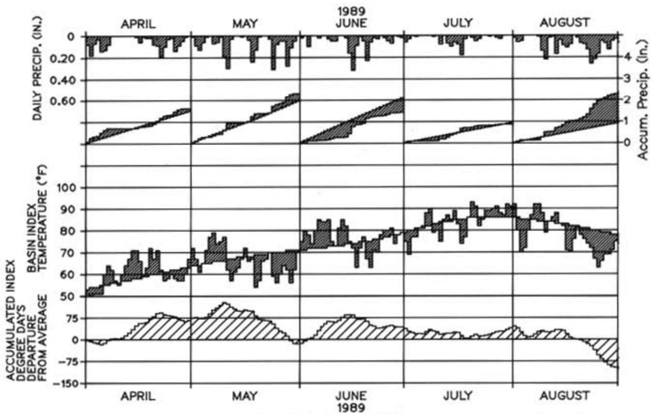
SNOWMELT SEASON Chart 4 Temperature and Precipitation Index 1988-1989 Columbia River Basin Above The Dalles, OR
