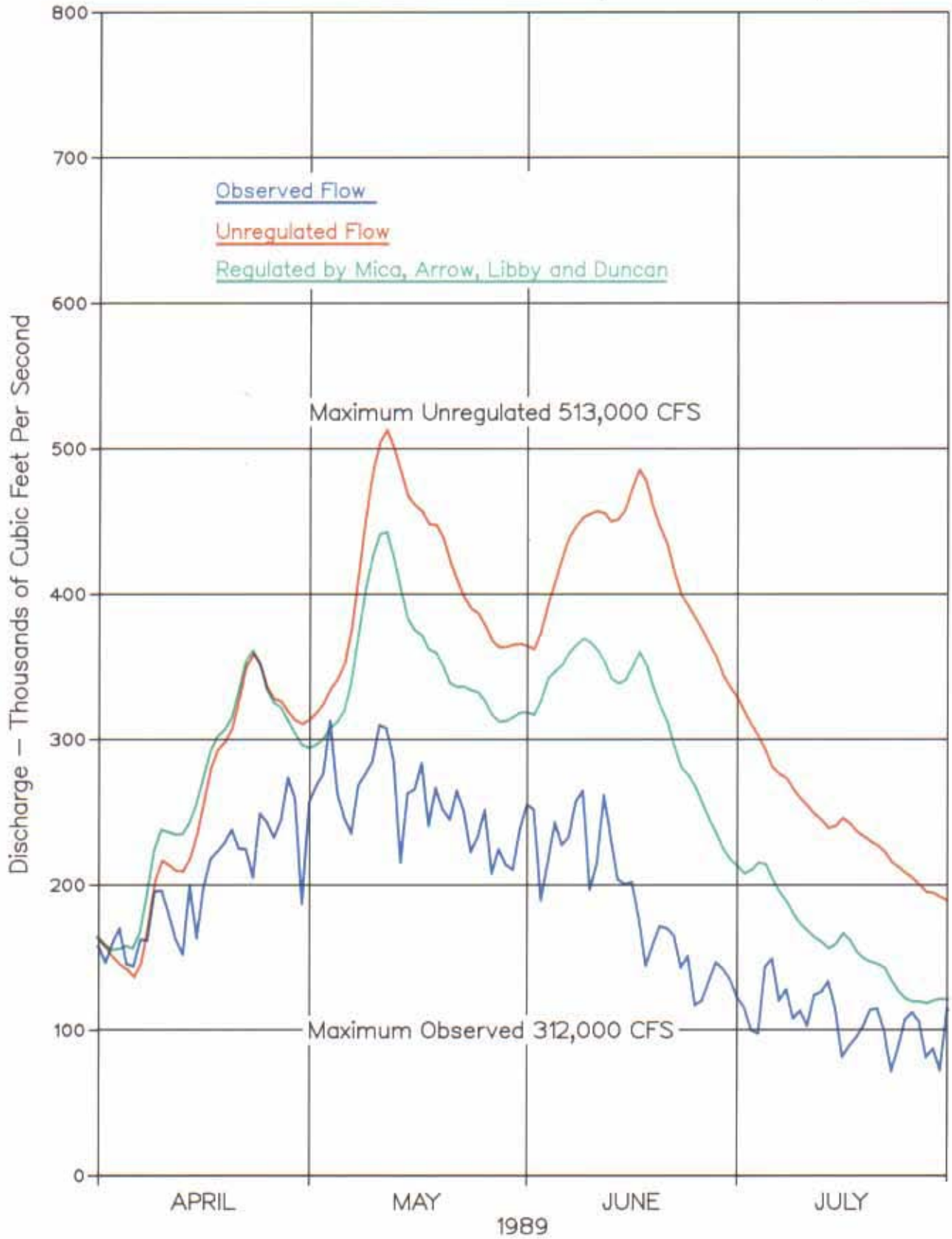
Chart 14 Columbia River at The Dalles 1 April 1989 - 31 July 1989
