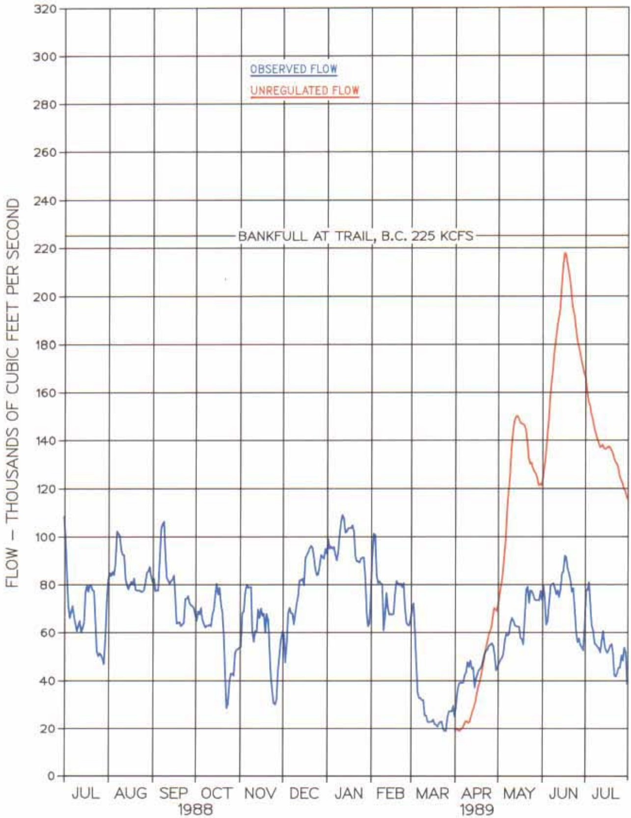
Chart 11 Columbia River at Birchbank 1 July 1988 – 31 July 1989
