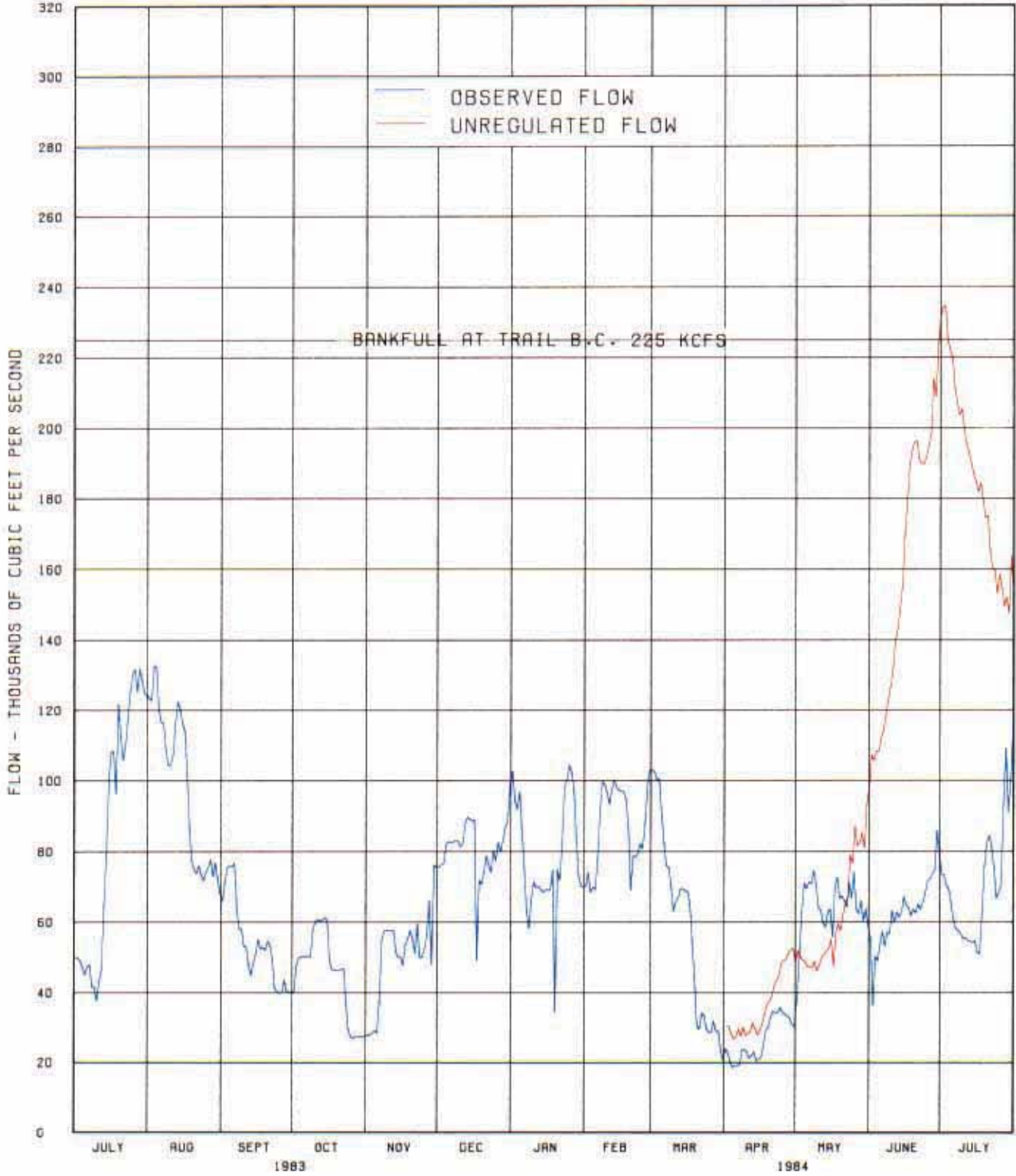
Chart 10 Columbia River at Birchbank 1 Jul 1983 - 31 Jul 1984
