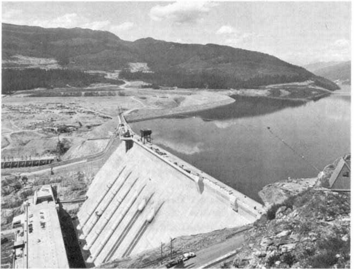
REVELSTOKE PROJECT. A summer 1984 view of B.C. Hydro's Revelstoke Project from the left bank of the Columbia River. The reservoir began filling on 11 October 1983 and reached its highest elevation of the year, 1877.8 ft, on 13 August 1984. Three generating units were in operation by 30 September 1984.
