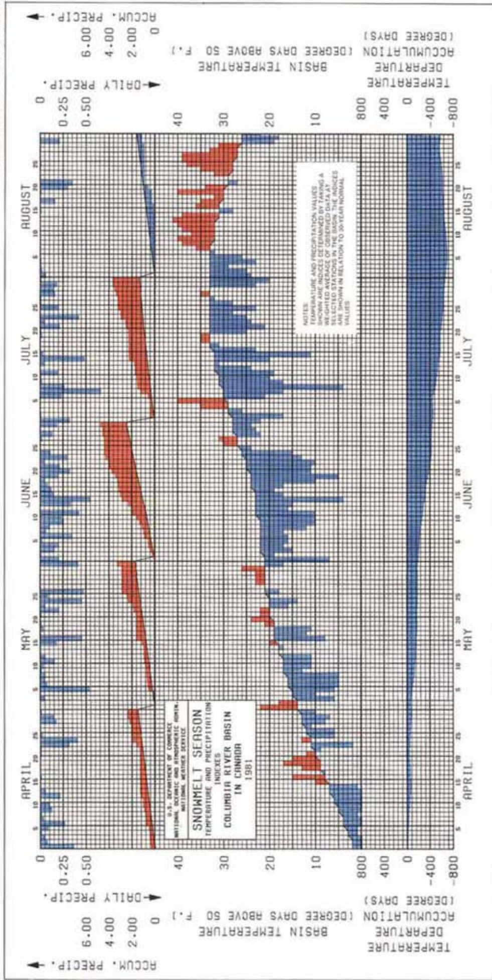
Chart 4 Snowmelt Season Temperature and Precipitation Indexes 1981 Columbia River Basin at Canada
