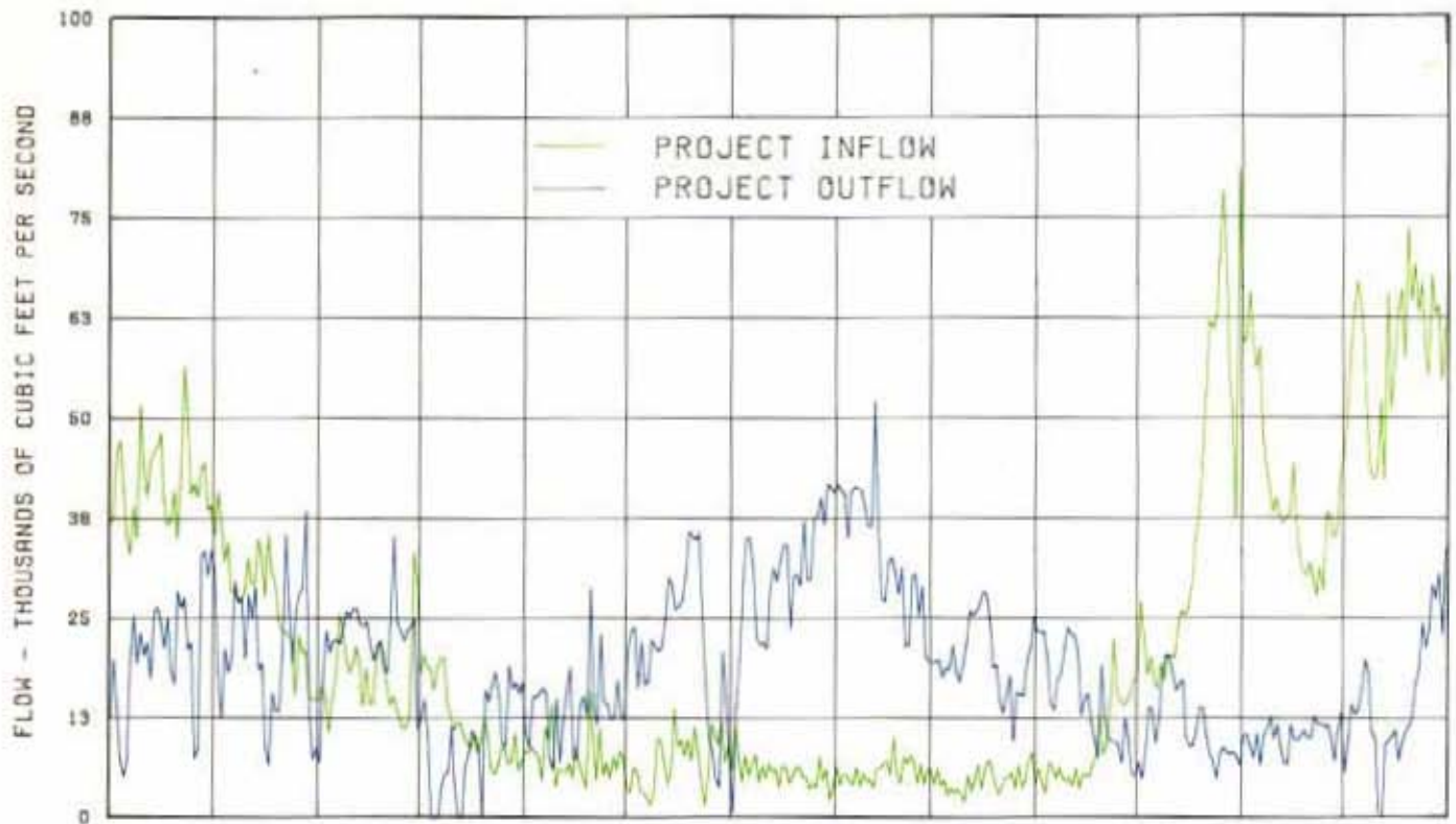
Chart 5 Regulation of Mica 1 July 1980 - 31 July 1981
