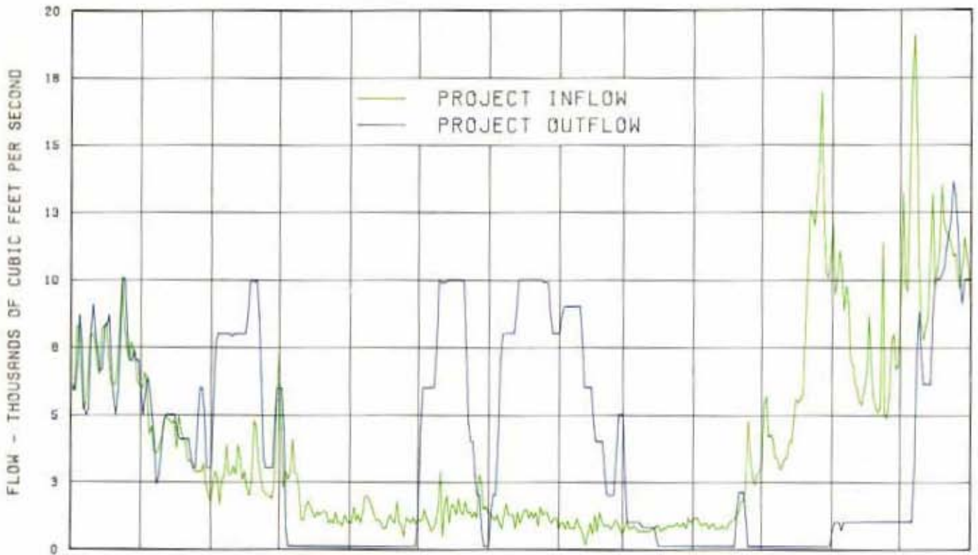
Chart 7 Regulation of Duncan 1 July 1980 - 31 July 1981
