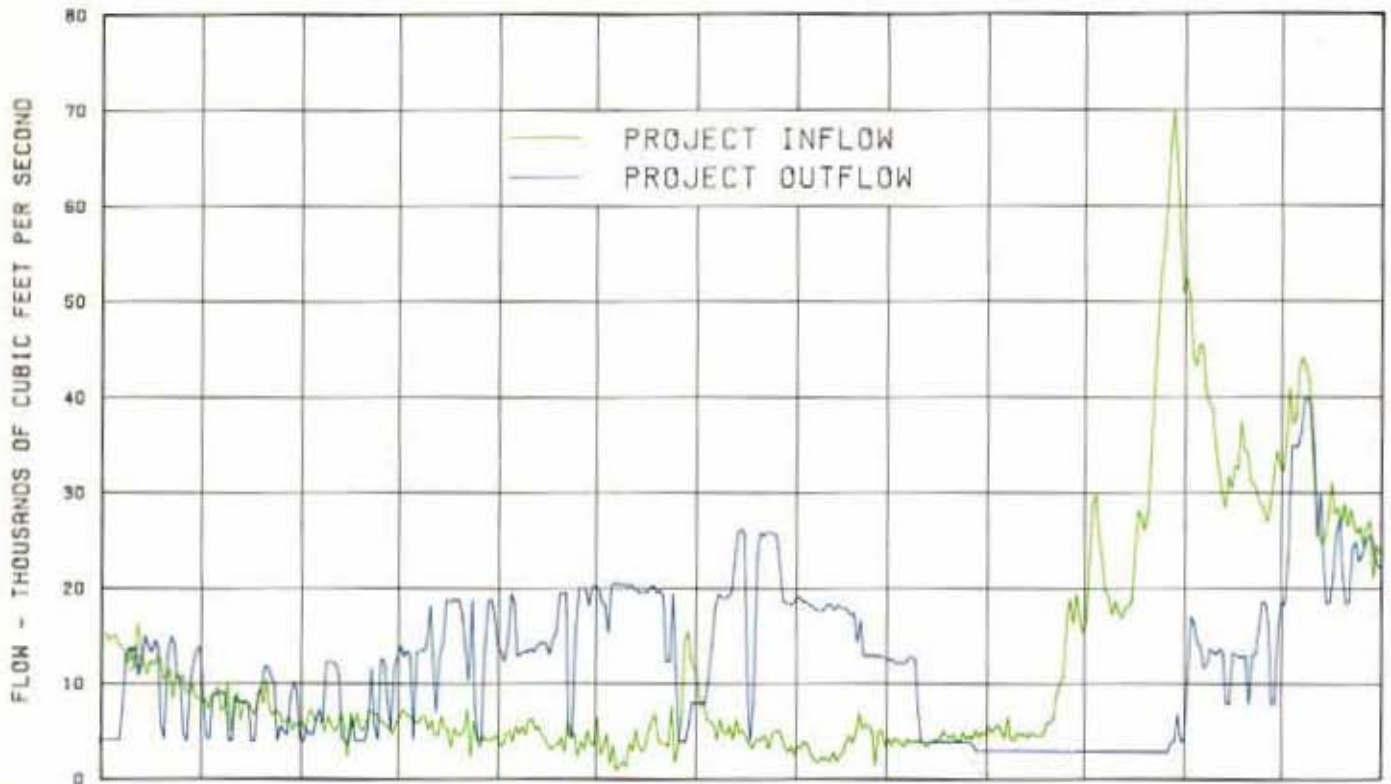
Chart 8 Regulation of Libby 1 July 1980 - 31 July 1981
