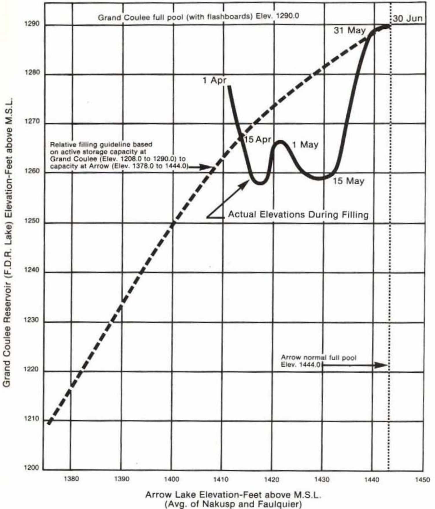
Chart 14 1981 Relative Filling Arrow and Grand Coulee
