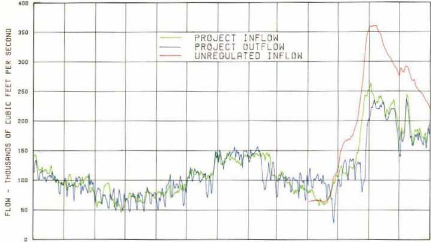
Chart 11 Regulation of Grand Coulee 1 July 1980 - 31 July 1981
