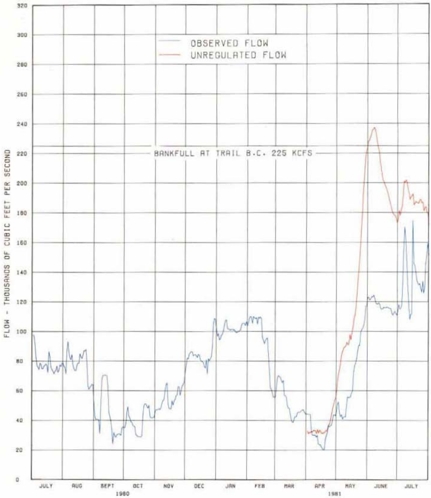
Chart 10 Columbia River at Birchbank 1 July 1980 - 31 July 1981
