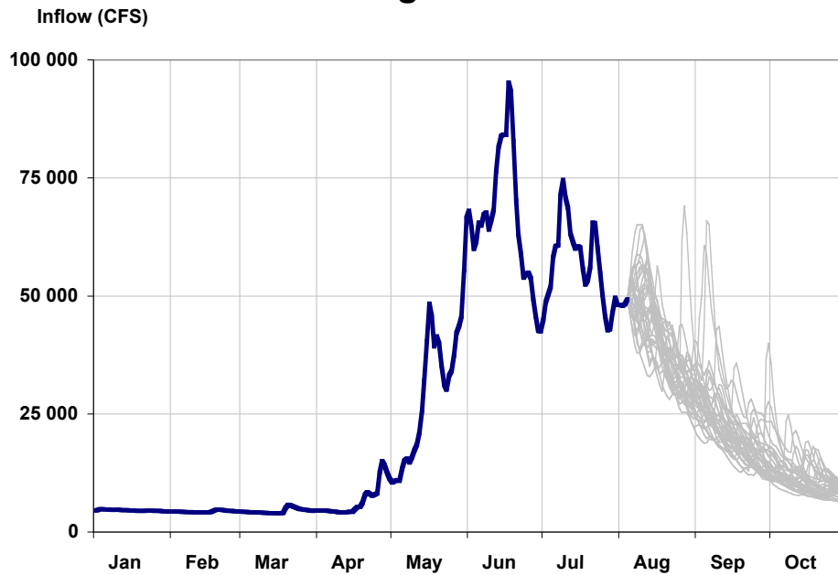
Figure 1 Series of synthetic hydrographs produced using the ESP forecasting procedure. Forecast date is 01 August in the example
