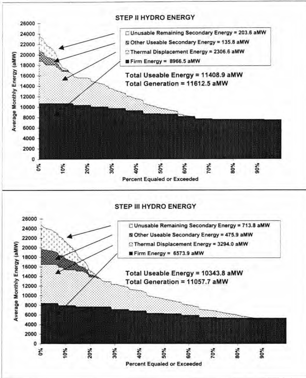
CHART 1 2001-02 DDBP STUDY DURATION CURVES OF 30 YEAR MONTHLY HYDRO GENERATION (aMW)
